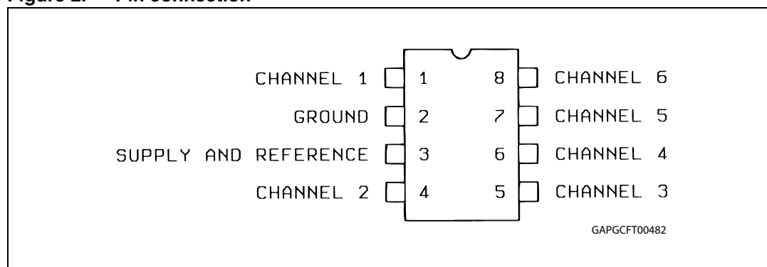
Figure 2. Pin connection
