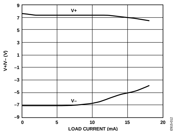
Figure 12. Charge Pump V+/- vs. Load Current ( V_{CC} = 3.3\text{ V} )
