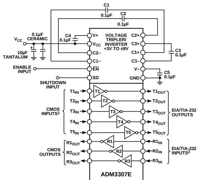
Figure 1. ADM3307E Functional Block Diagram
