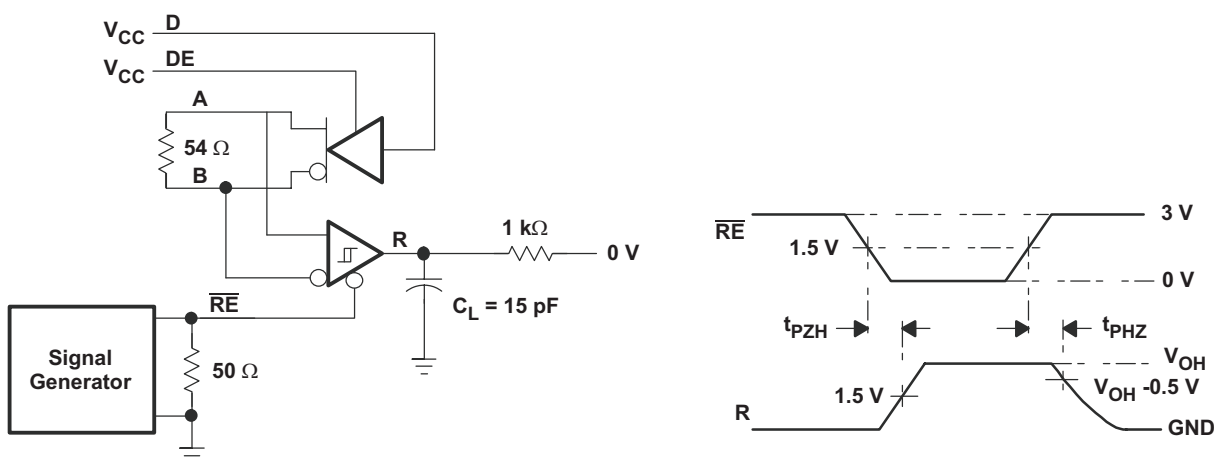
Figure 10. Receiver Enable/Disable Test Circuit and Waveforms, Data Output High
