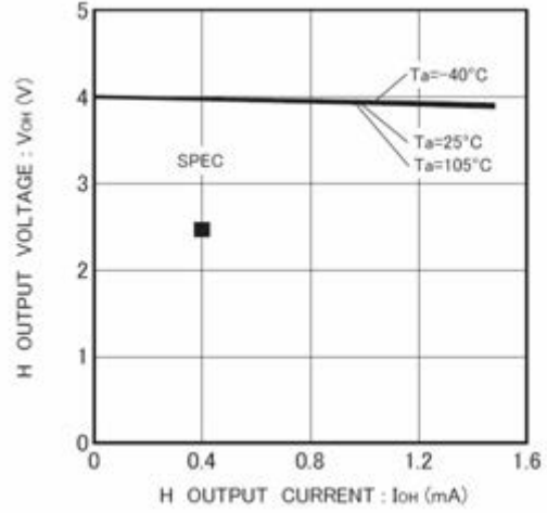
Figure 6. H output voltage V_{OH} - I_{OH} ( V_{CC}=4.0\text{V} )
