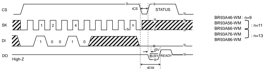
Figure 32. Chip erase cycle timing
