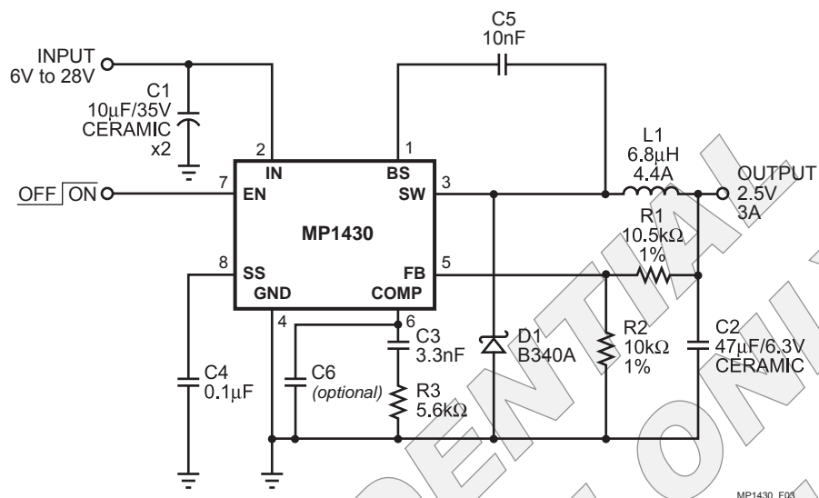
Figure 3—MP1430 with AVX 47μF, 6.3V Ceramic Output Capacitor
