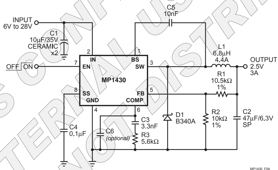
Figure 4—MP1430 with Panasonic 47μF, 6.3V Special Polymer Output Capacitor
