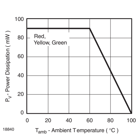
Figure 1. Power Dissipation vs. Ambient Temperature
