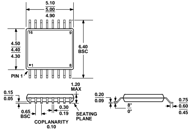
Figure 40. 16-Lead Thin Shrink Small Outline Package [TSSOP] (RU-16) Dimensions shown in millimeters
