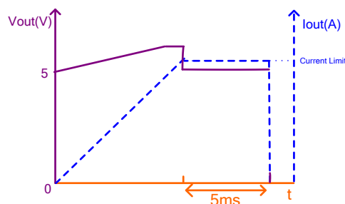
Figure 6: Over-Current Limit
