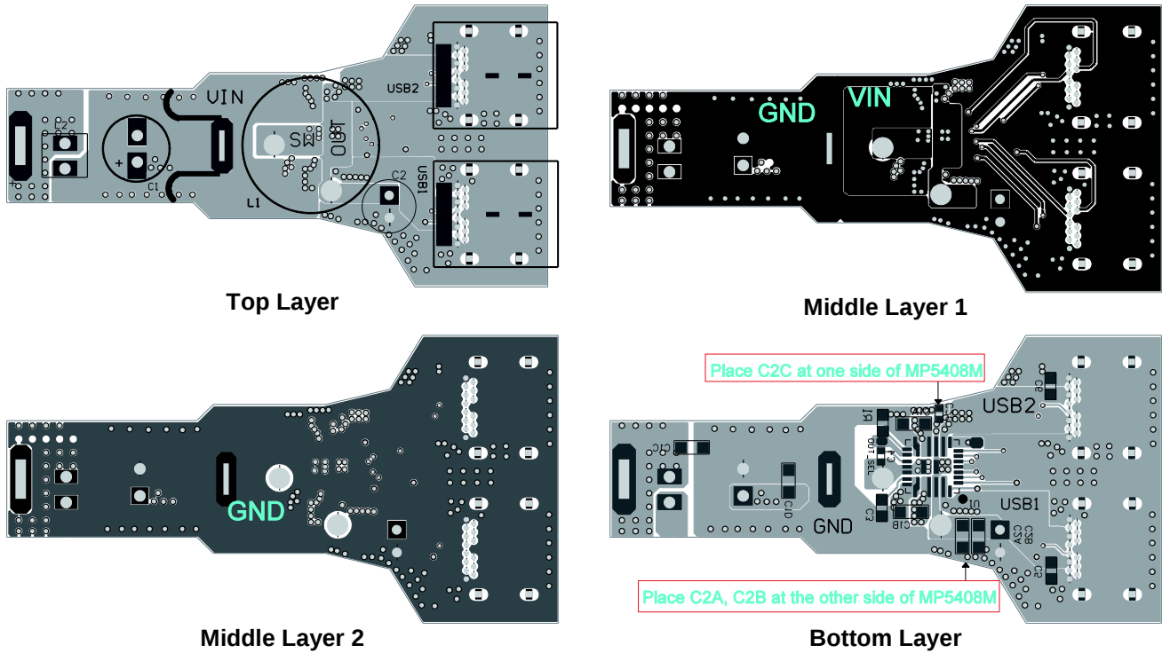
Figure 11: Recommended Layout
