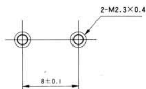
PCB Mounting Pattern
