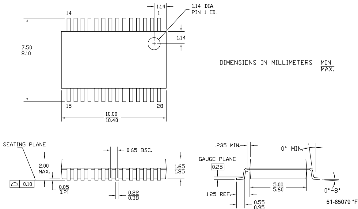
Figure 16. 28-pin (210-mil) SSOP Package Outline
