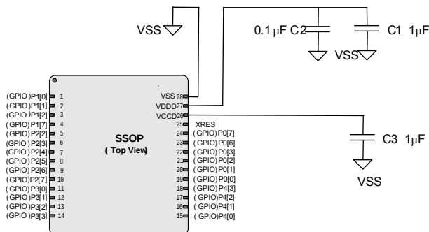
Figure 15. 28-SSOP Example
