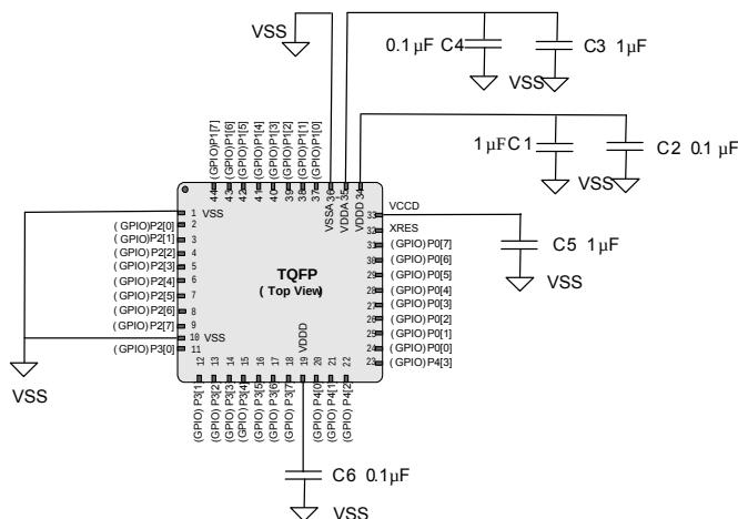
Figure 13. 44-TQFP Package Example
