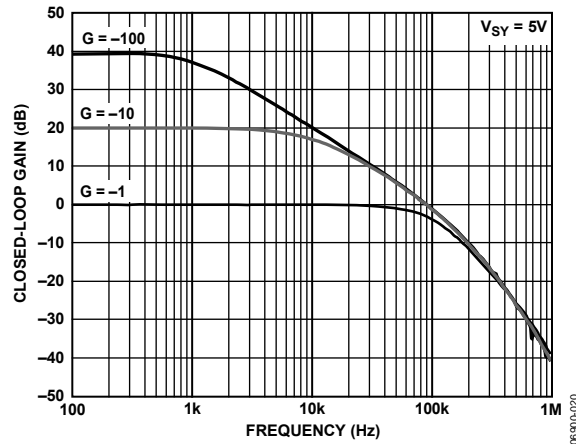
Figure 29. Closed-Loop Gain vs. Frequency
