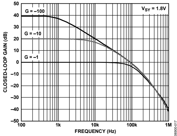
Figure 26. Closed-Loop Gain vs. Frequency
