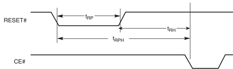
Figure 13.1 Reset Timings
