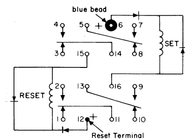
CODE 6 Dual Diode
