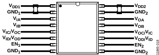
Figure 29. Recommended Printed Circuit Board Layout, QSOP
