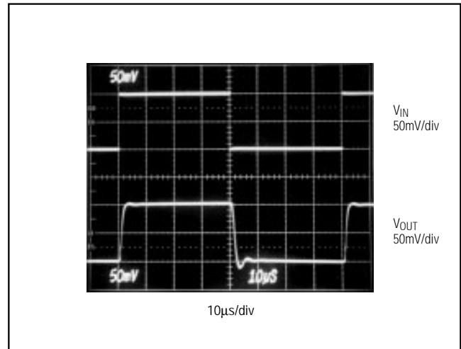
Figure 9b. Driving a 10,000pF Capacitive Load with a 47 \Omega Isolation Resistor
