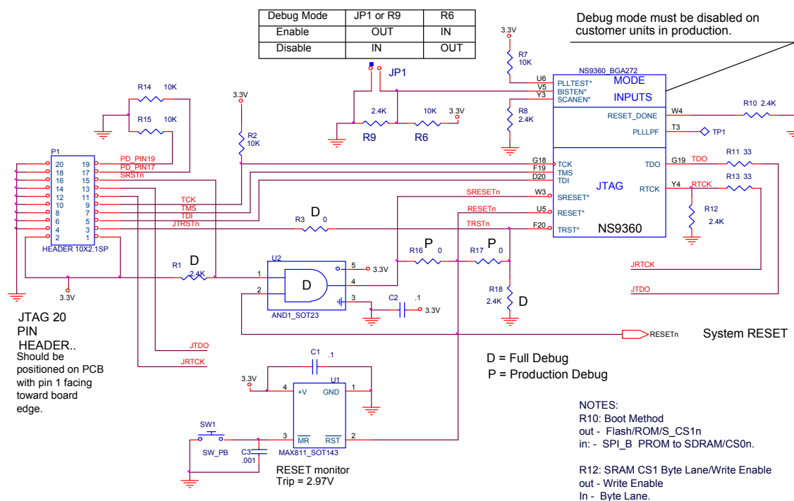
Figure 6: JTAG interface
