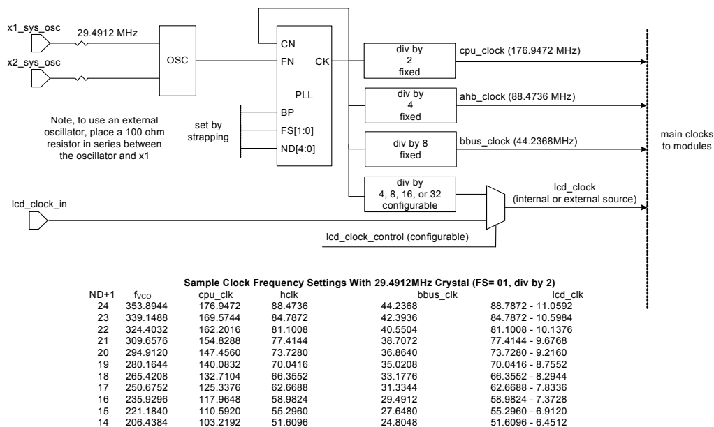
Figure 3: NS9360 system clock generation (PLL)
