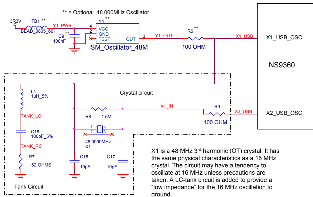
Figure 4: USB clock
