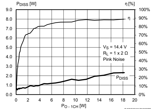
Figure 7. Efficiency and power dissipation ( V_S = 14.4\text{ V} , R_L = 1 \times 2\ \Omega , f = 1\text{ kHz} pink noise)
