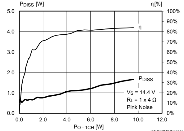
Figure 5. Efficiency and power dissipation ( V_S = 14.4\text{ V} , R_L = 1 \times 4\ \Omega , f = 1\text{ kHz} pink noise)
