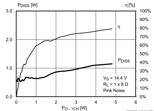
Figure 9. Efficiency and power dissipation ( V_S = 14.4\text{ V} , R_L = 1 \times 8\ \Omega , f = 1\text{ kHz} pink noise)
