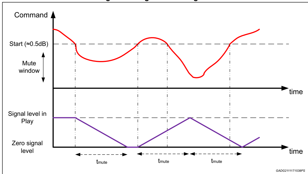
Figure 41. Digital-Mute diagram
