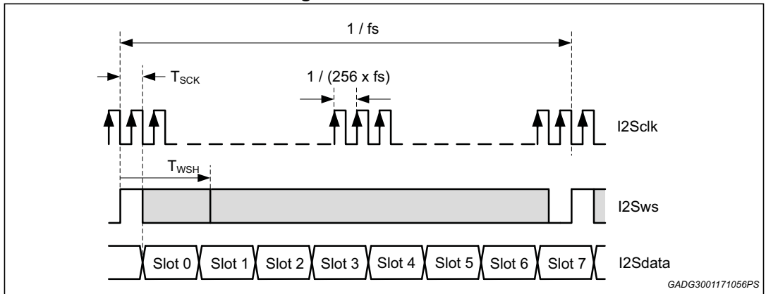
Figure 66. TDM8 mode
