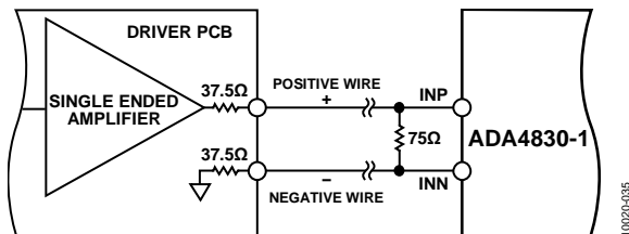
Figure 22. Pseudo Differential Mode with Balanced Source Impedance
