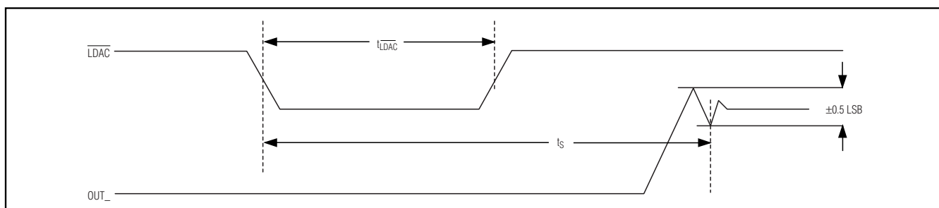
Figure 3. \overline{LDAC} Timing
