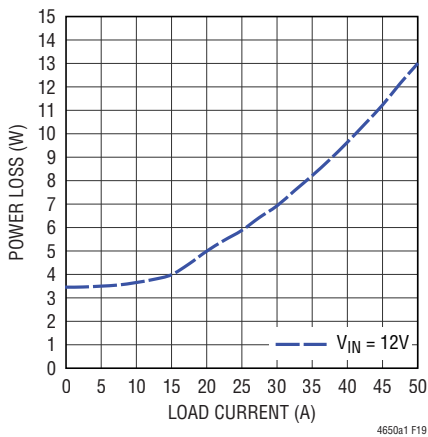
Figure 19. 5V OUT Power Loss Curve
