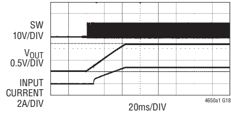
Single Phase Start-up with 25A Load
