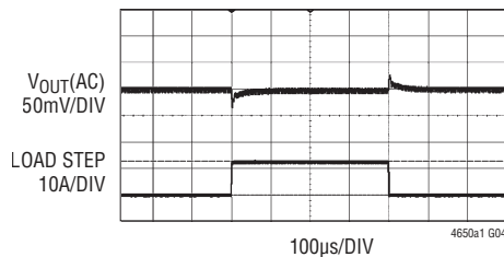
1V Dual Phase Single Output Load Transient Response (Ceramic Output Capacitor Only)
