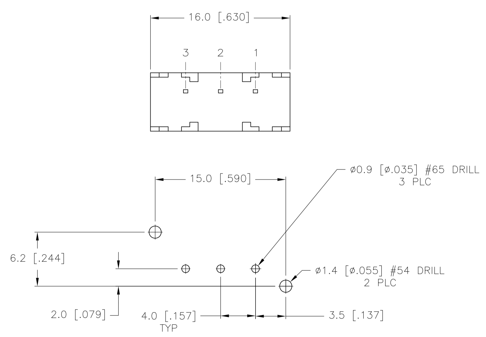
RECOMMENDED BOARD LAYOUT PC LAYOUT TOLERANCE: ±.002
