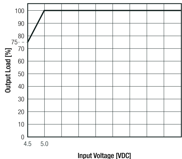
Line Derating
