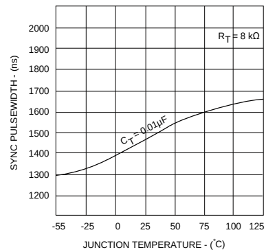
Figure 16 • Sync Pulsewidth Vs. Temperature
