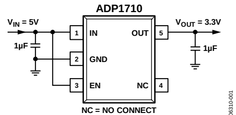
Figure 1. ADP1710 with Fixed Output Voltage, 3.3 V
