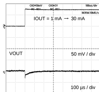
Fig.20 Load Response (Co = 2.2 μF) (BH30NB1WHFV)
