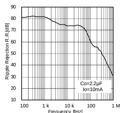
Fig.18 Ripple Rejection (BH33NB1WHFV)
