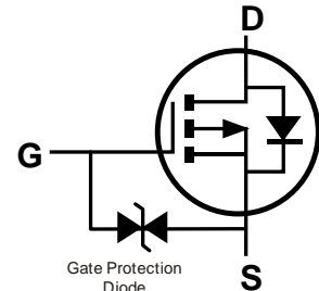
Internal Schematic
