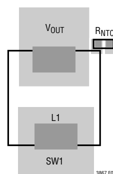
Figure 8. Thermistor Location. Place Thermistor Next to Inductor for Accurate Sensing of the Inductor Temperature, But Keep the ITEMP Pin Away from the Switch Nodes and Gate Drive Traces
