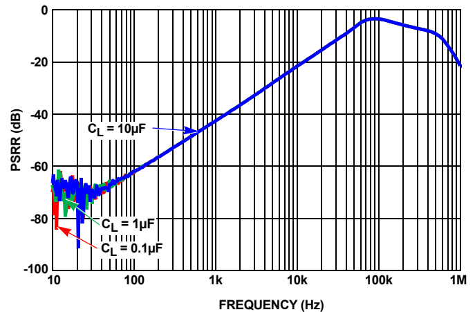
FIGURE 99. RIPPLE REJECTION AT DIFFERENT CAPACITIVE LOADS
