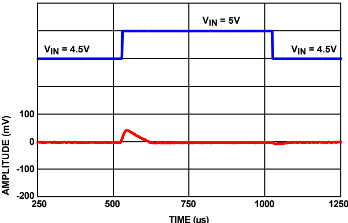
FIGURE 110. LINE TRANSIENT RESPONSE WITH 10\mu F LOAD
