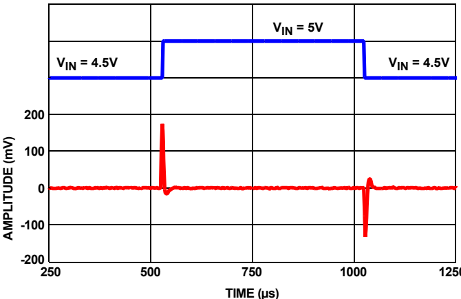
FIGURE 109. LINE TRANSIENT WITH 0.1\mu F LOAD
