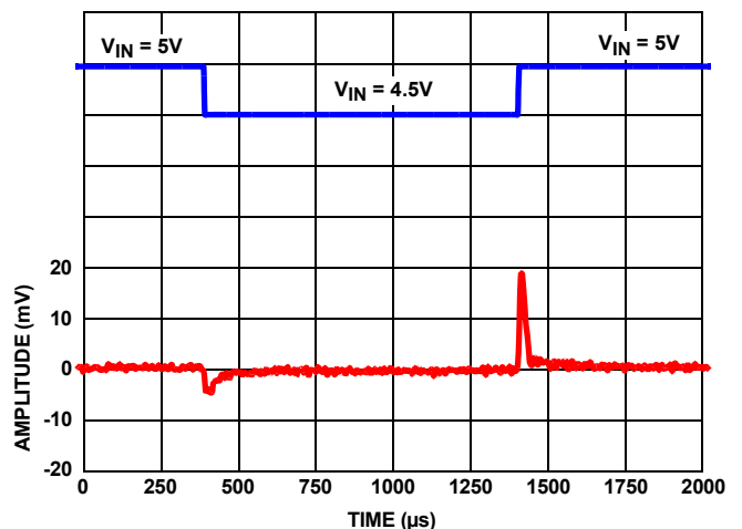
FIGURE 8. LINE TRANSIENT RESPONSE WITH 10μF LOAD
