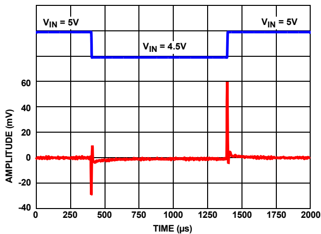
FIGURE 7. LINE TRANSIENT RESPONSE WITH 0.22μF LOAD
