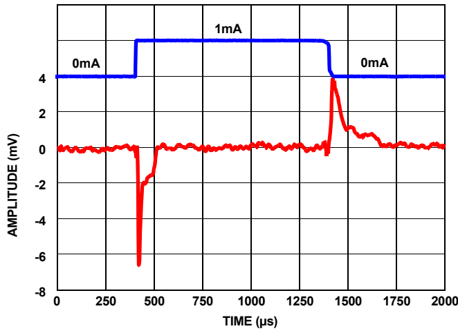
FIGURE 79. LOAD TRANSIENT RESPONSE AT 1mA LOAD AT 1µF
