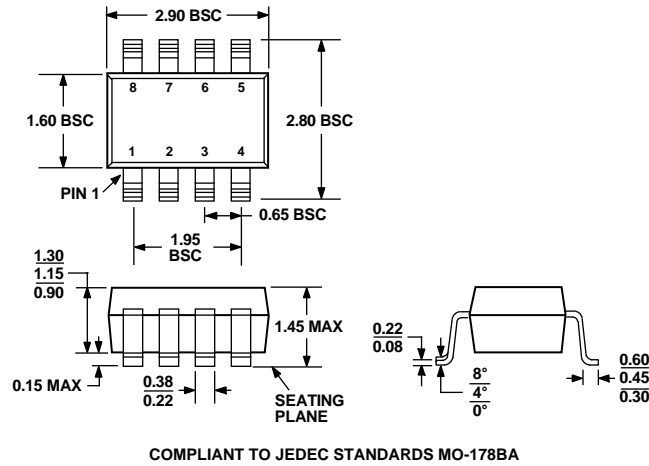
Figure 43. 8-Lead Small Outline Transistor Package [SOT-23] (RT-8)
