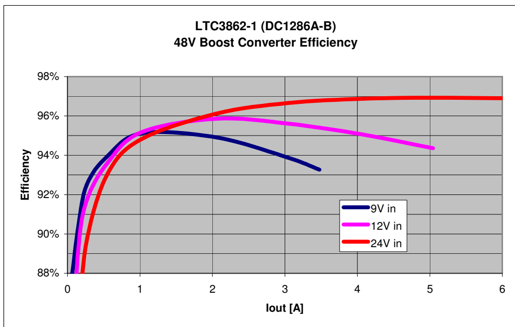
Figure 4. DC1286A-B Efficiency
