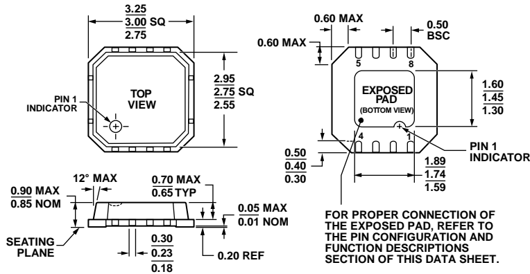
Figure 55. 8-Lead Lead Frame Chip Scale Package [LFCSP_VD] 3 mm x 3 mm Body, Very Thin, Dual Lead (CP-8-2)
