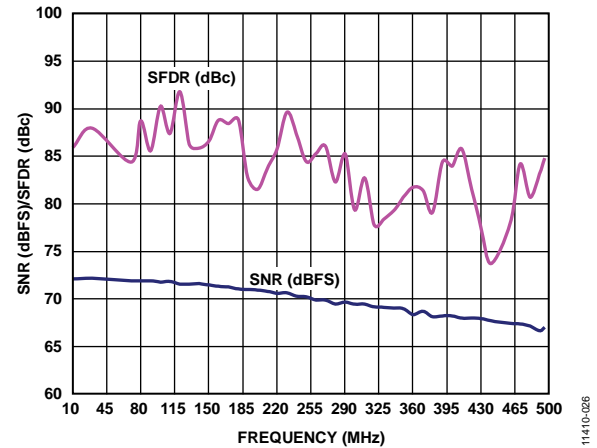
Figure 26. AD9683-250 Single-Tone SNR/SFDR vs. Input Frequency ( f_{IN} ), RFLCK = 1.0 GHz with Divide by 4 (Address 0x09 = 0x21)
