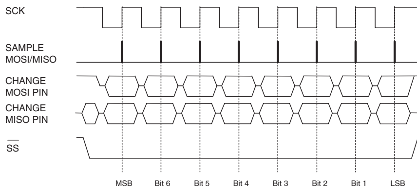
Figure 8-1. Data Byte Exchange – Signals
