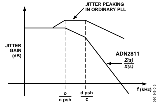
Figure 13. Jitter Response vs. Conventional PLL
