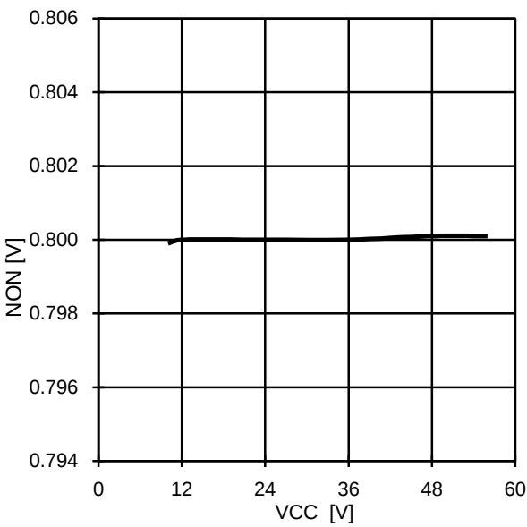
Fig.14 Reference Voltage-VCC
