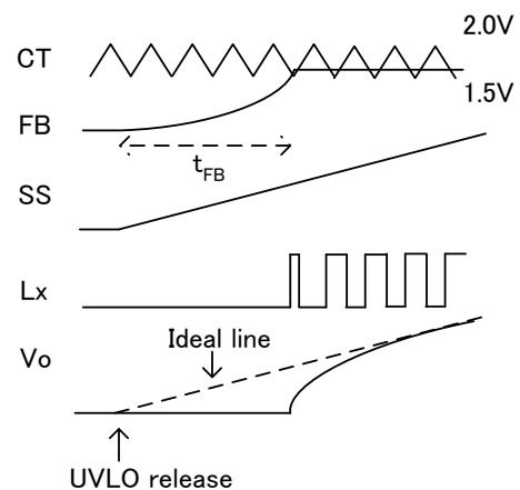
Fig.58 Startup Timing Chart
