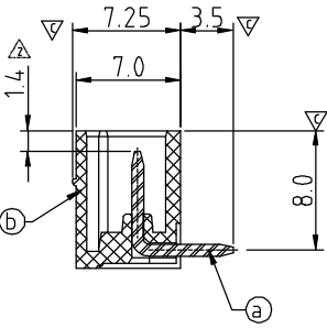
SECTION P-P
