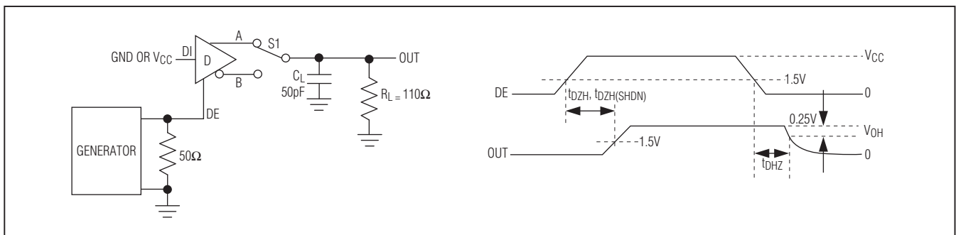
Figure 4. Driver Enable and Disable Times ( t_{DZH} , t_{DZH} )
