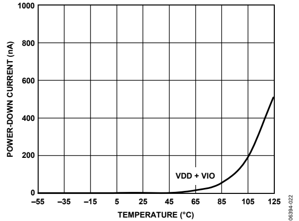
Figure 22. Power-Down Currents vs. Temperature
