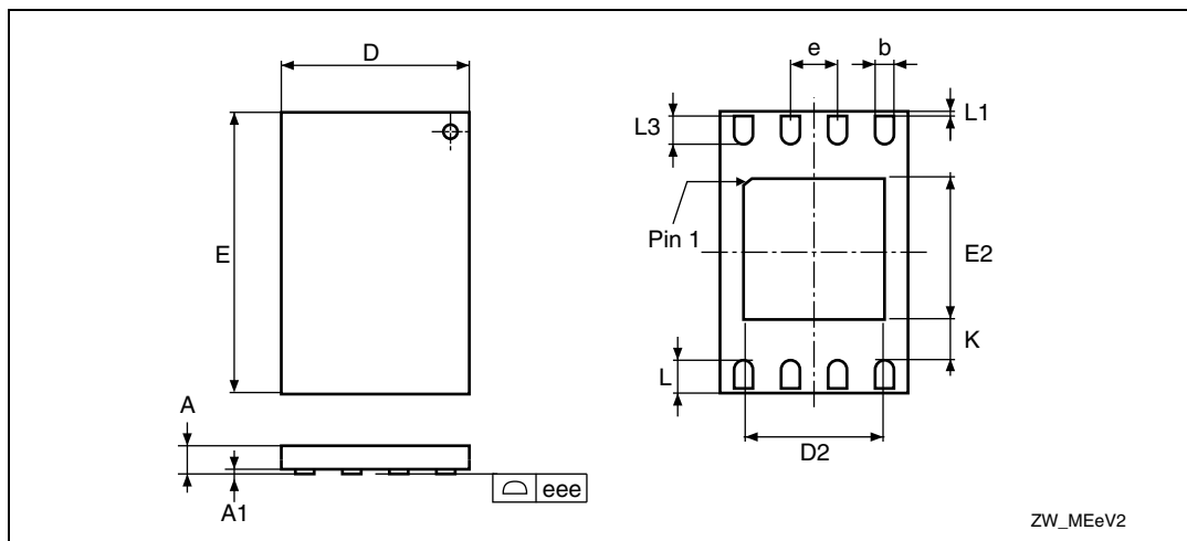
Figure 17. UDFPN8 (MLP8) - 8-lead ultra thin fine pitch dual flat no lead, package outline
