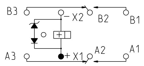
TERMINAL VIEW
