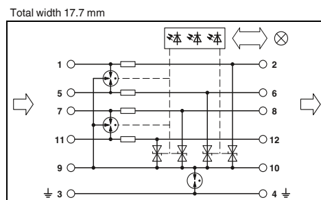
4-wire with common reference potential, 9/10 connection grounded via gas-filled surge
