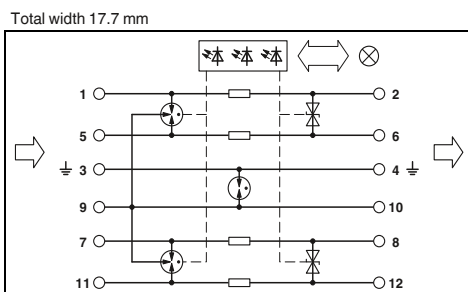
2 double conductors (loops), floating, 9/10 connection grounded via gas-filled surge
