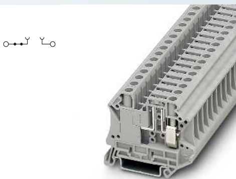
6 (10) mm 2 , 20 A, disconnect terminal block, with test socket screws
