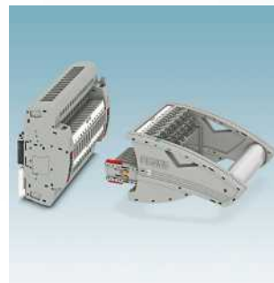
FAME plug-in test system with screw connection, VDE types, for wall and DIN rail mounting
